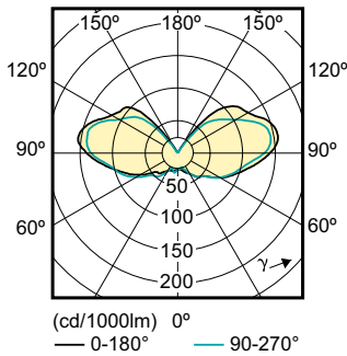
Light Distribution Diagram - LED 10W G4 WH 12V ND 1BC/6
