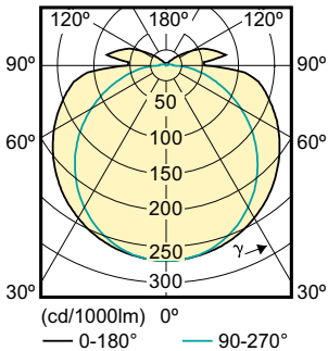
Light Distribution Diagram - 16.5T8/24-3500 IF-6U 10/1
