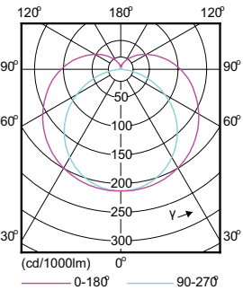
Light Distribution Diagram - 10T8/48-3500 IF 10/1
