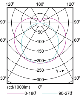
Light Distribution Diagram - 10T8/48-4000 IF 10/1
