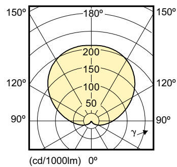
Light Distribution Diagram - CorePro LEDbulb 15-100W 827 E27
