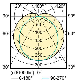
Light Distribution Diagram - MAS LEDtube VLE 600mm 10W865 T8C ROT
