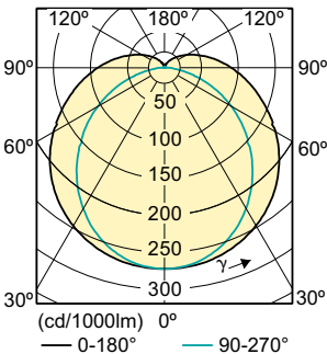
Light Distribution Diagram - MAS LEDtube STD 600mm 10W865 T8 I
