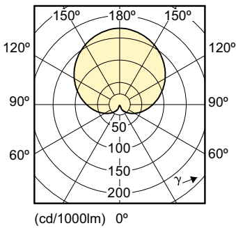
LEDbulb, Bulb A19 13W-100W 5000K 1500lm
