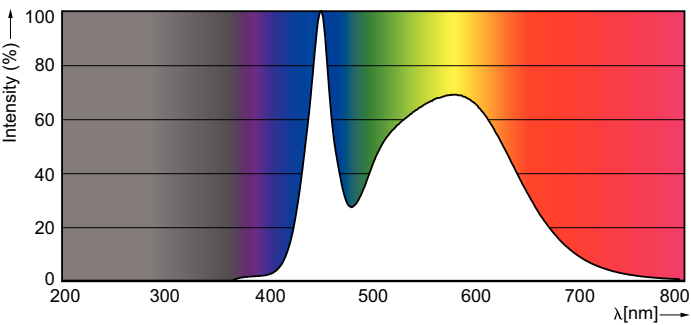
LEDbulb, Bulb A19 13W, 19W 5000K
