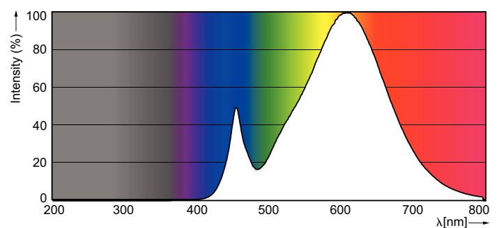
Spectral Power Distribution Colour - MAS LEDlustre DT 4-25W E14 P48 CL
