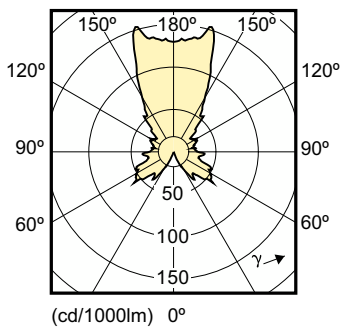
Light Distribution Diagram - MAS LEDlustre DT 4-25W E14 P48 CL
