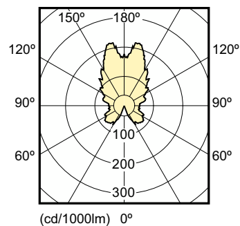
Light Distribution Diagram - MAS LEDcandle DT 6-40W B15 B38 CL
