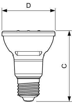
LED D 5.5-50W E27 2700K PAR20 40D
