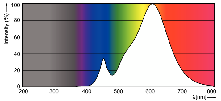
Spectral Power Distribution Colour - CorePro LEDspotLV 5.5-35W 827 MR16 36D
