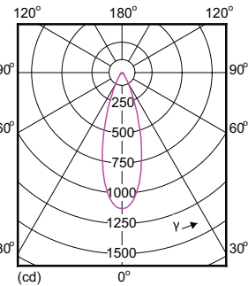
Light Distribution Diagram - MASTER LED 5.5-50W 3000K MR16 36D
