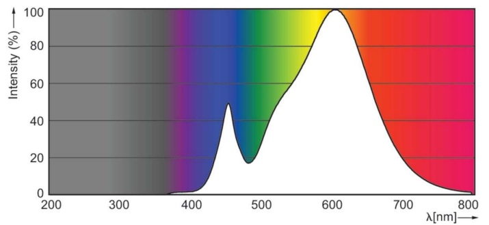
Spectral Power Distribution Colour - MASTER LED 4-35W 3000K MR16 24D
