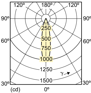
Light Distribution Diagram - MASTER LED 4-35W 3000K MR16 24D CN
