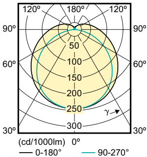
Light Distribution Diagram - MAS LEDtube 1500mm UO 25W 865 T8
