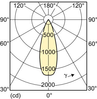
Light Distribution Diagram - 8.5MRX16/F35 2700 DIM AF 10/1
