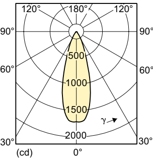
Light Distribution Diagram - MAS LEDspotLV D 8.0-50W 830 MR16 36D
