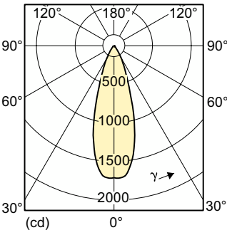
Light Distribution Diagram - 8.5MRX16/F35 3000 DIM AF 10/1
