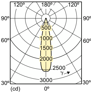
Light Distribution Diagram - 7MR16/LED/F25/840/DIM AF2 10/1
