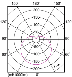
Light Distribution Diagram - SceneSwitch Color A60 9.5-70W E27 WW/CDL
