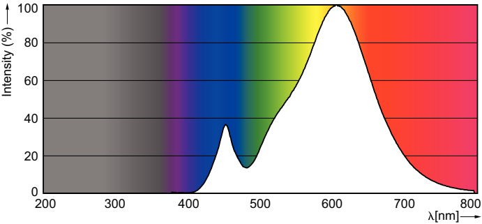
Spectral Power Distribution Colour - ESS LEDCandle 25W B35 E14 WW FR ND TRK
