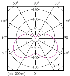
Light Distribution Diagram - ESS LEDCandle 25W B35 E14 WW FR ND TRK
