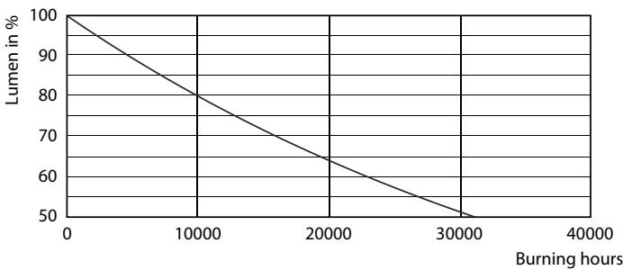
Lumen Maintenance Diagram - ESS LEDCandle 25W B35 E14 WW FR ND TRK
