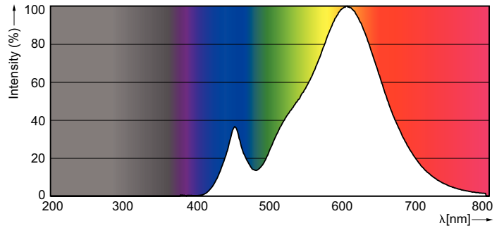
SDPO_LEDLSR_0003-Spectral Power distribution
