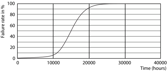
Life Expectancy Diagram - ESS LEDCandle 40W B35 E14 WW FR ND TRK
