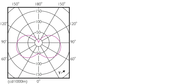
Light Distribution Diagram - ESS LEDCandle 40W B35 E14 WW FR ND TRK
