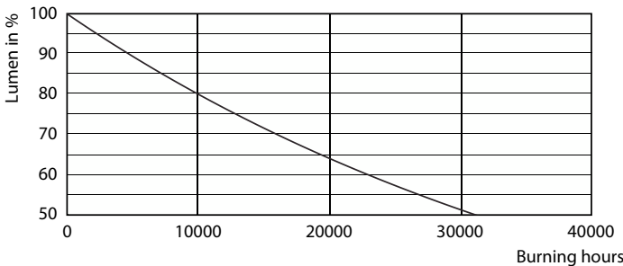
Lumen Maintenance Diagram - ESS LEDCandle 40W B35 E14 WW FR ND TRK
