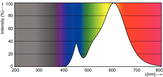
Spectral Power Distribution Colour - ESS LEDCandle 40W B35 E14 WW FR ND TRK
