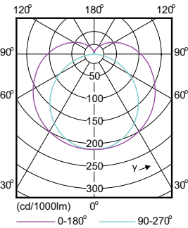
Light Distribution Diagram - 15T8/48-3500 IF 10/1
