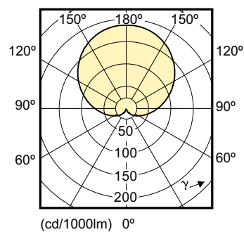
Light Distribution Diagram - CorePro LEDbulb D 11.5-75W 827 E27
