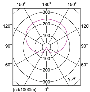
Light Distribution Diagram - LEDBulb 4-40W E27 6500K 220V P45 2BC
