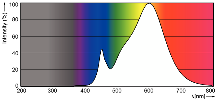
Spectral Power Distribution Colour - CorePro LEDbulb ND 5.5-40W A60 E27 830
