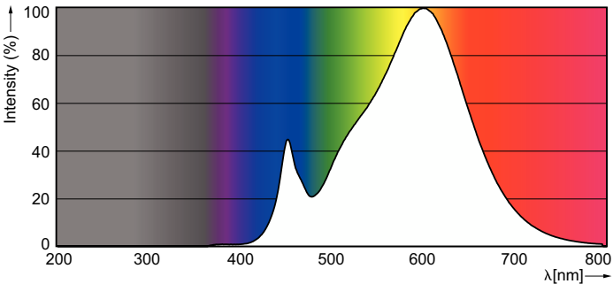
Spectral Power Distribution Colour - LEDBulb 9.5-70W E27 830 220-240V 1PF/10
