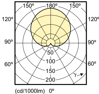
Light Distribution Diagram - LEDBulb 9.5-70W E27 830 220-240V 1PF/10
