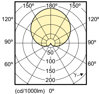
Light Distribution Diagram - LEDBulb 9.5-70W E27 830 220-240V 1BL/4
