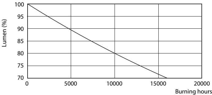
Lumen Maintenance Diagram - CorePro LEDbulb 10.5-75W 830 E27
