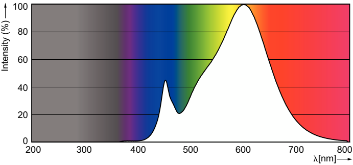
Spectral Power Distribution Colour - CorePro LEDbulb 10.5-75W 830 E27
