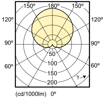
Light Distribution Diagram - CorePro LEDbulb 10.5-75W 830 E27
