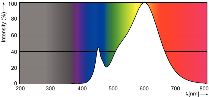
Spectral Power Distribution Colour - LEDBulb 10.5-85W E27 830 220-240V 1PF/10
