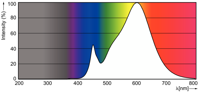
Spectral Power Distribution Colour - LEDBulb 13-100W E27 830 220-240V 1PF/12
