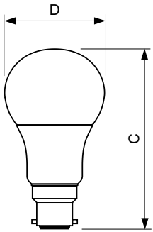
Basic Bulb 10.5W-75W 1055lm 3000K B22 ND
