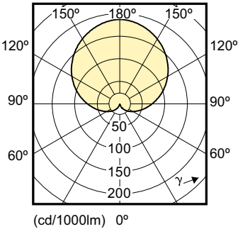
Light Distribution Diagram - LEDBulb 10.5-85W E27 865 220-240V 2BL/4
