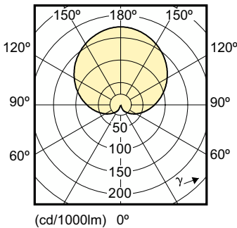
Light Distribution Diagram - LEDBulb 13-100W E27 865 220-240V 2BL/4
