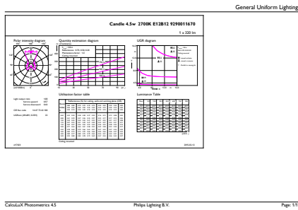
General uniform lighting - 4.5B12/LED/827-22/E12/DIM 120V
