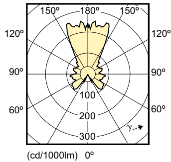
Light Distribution Diagram - 4.5B12/LED/827-22/E12/DIM 120V
