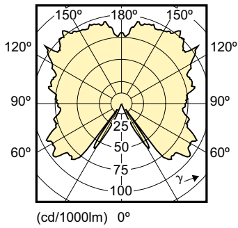
Light Distribution Diagram - 7A15/LED/827-22/E26/CL/DIM 120V
