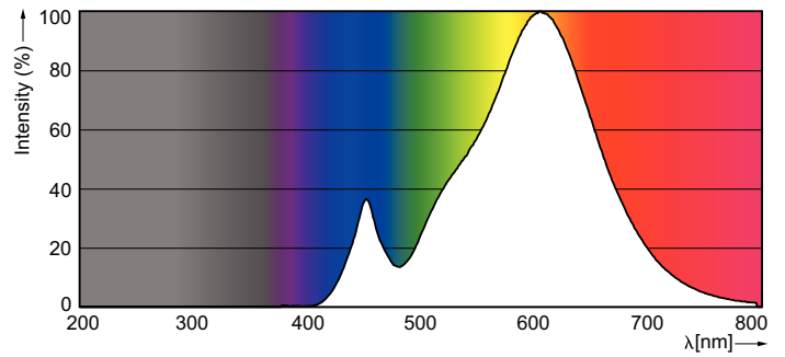
Spectral Power Distribution Colour - 7A15/LED/827-22/E26/CL/DIM 120V
