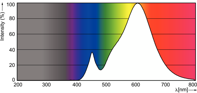
Spectral Power Distribution Colour - 4B11/827 E12 8/1
