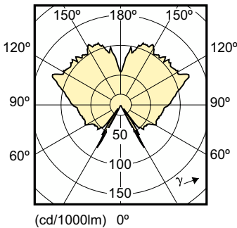
Light Distribution Diagram - 4B11/827 E12 8/1
