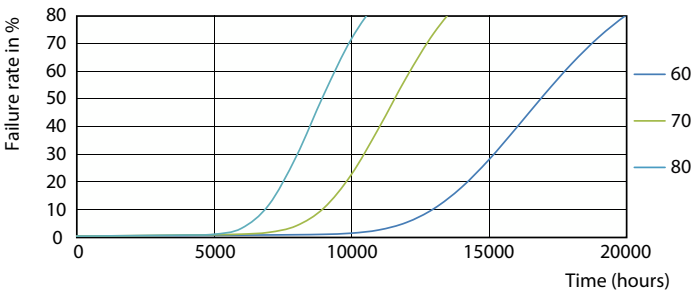
Life Expectancy Diagram - LEDtube 1200mm 16W 740 T8 AP I G
