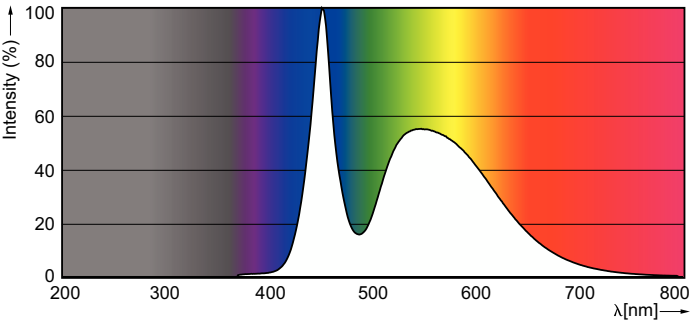
Spectral Power Distribution Colour - LEDtube 1200mm 16W 765 G HV
