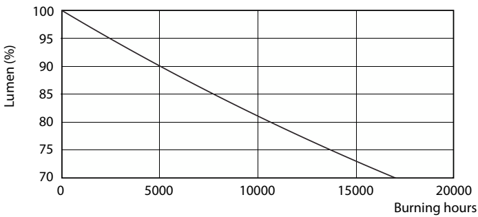
Lumen Maintenance Diagram - LEDtube 1200mm 16W 765 G HV
