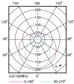
Light Distribution Diagram - LEDtube 1200mm 16W 765 G HV
