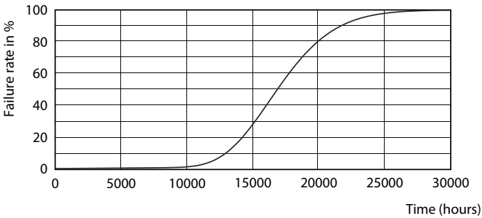
Life Expectancy Diagram - LEDtube 1200mm 16W 765 G HV
