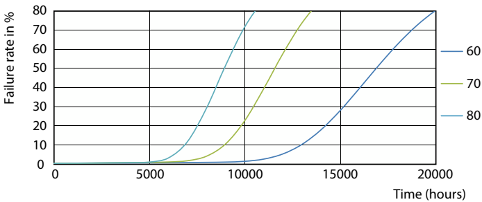
Life Expectancy Diagram - LEDtube 600mm 8W 740 G HV
