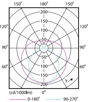
Light Distribution Diagram - LEDtube 600mm 8W 740 G HV
