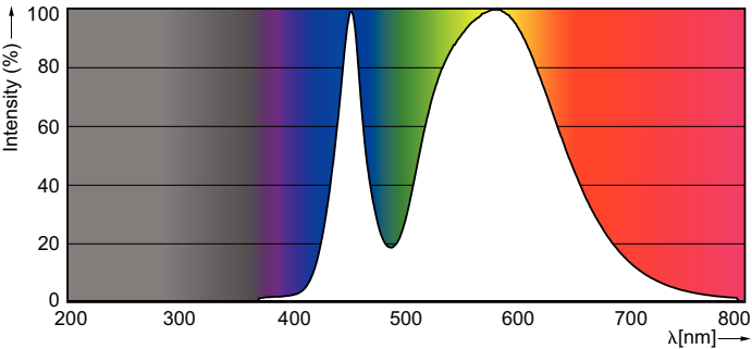
Spectral Power Distribution Colour - LEDtube 600mm 8W 740 G HV
