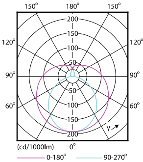
Light Distribution Diagram - LEDtube 600mm 8W 765 G HV
