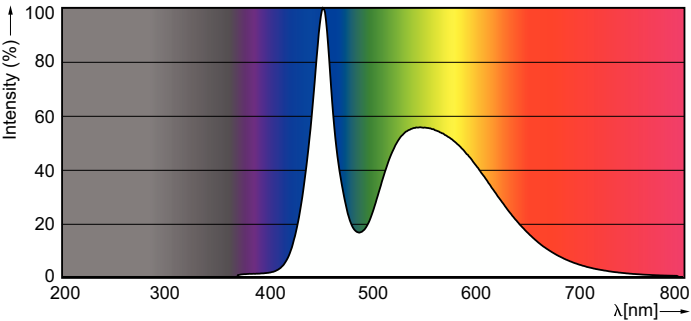
Spectral Power Distribution Colour - LEDtube 600mm 8W 765 G HV
