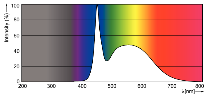
LEDtube 1200mm 18 W /865 T8 I W
