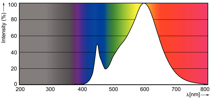
Spectral Power Distribution Colour - LEDBulb 9-60W E27 3000K W A19 4PK MX
