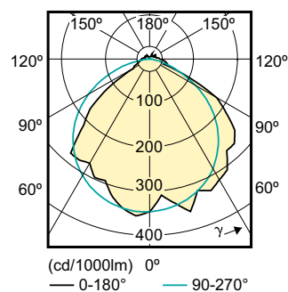
Light Distribution Diagram - MAS LEDtube 1200mm HO 18W840 T8 CLEAR
