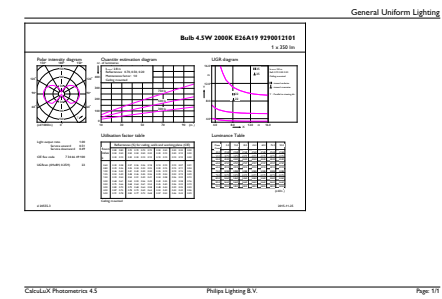
LEDlamps, LEDFilament 4.5-40W A19 Amber 2000K 350lm
