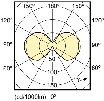
Light Distribution Diagram - 4.5A19b/LEDFilament/820/CL-A/DIM 120V
