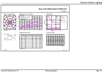
General uniform lighting - 4.5A19b/LEDFilament/820/CL-A/DIM 120V
