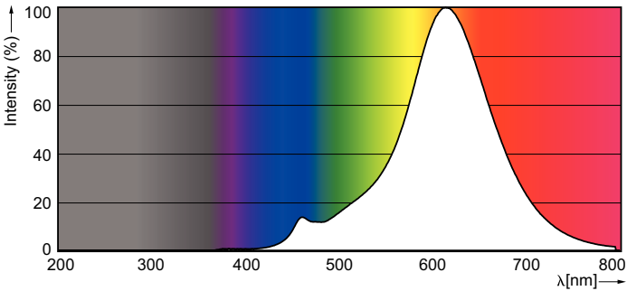
Spectral Power Distribution Colour - 4.5A19b/LEDFilament/820/CL-A/DIM 120V
