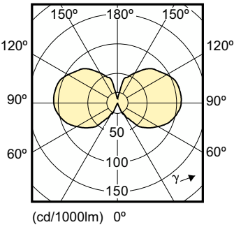
Light Distribution Diagram - BC5.5/ST19/LEDFilament/820/CL-A/DIM 120V
