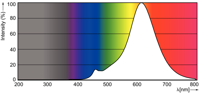
Spectral Power Distribution Colour - BC5.5/ST19/LEDFilament/820/CL-A/DIM 120V
